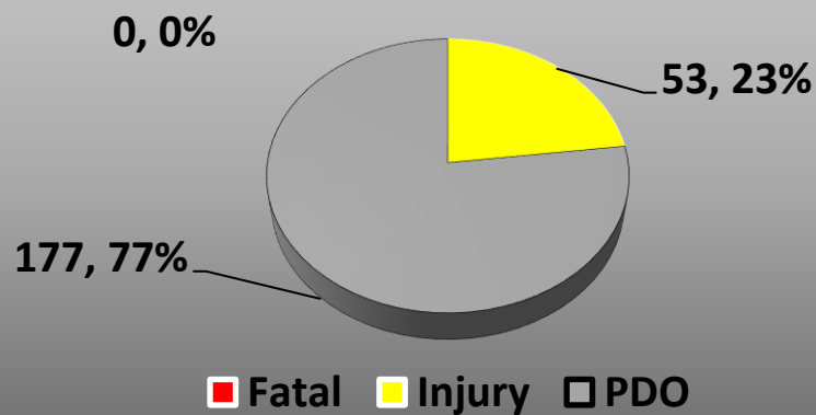
2018 Combined Monthly Total Crashes by Type
