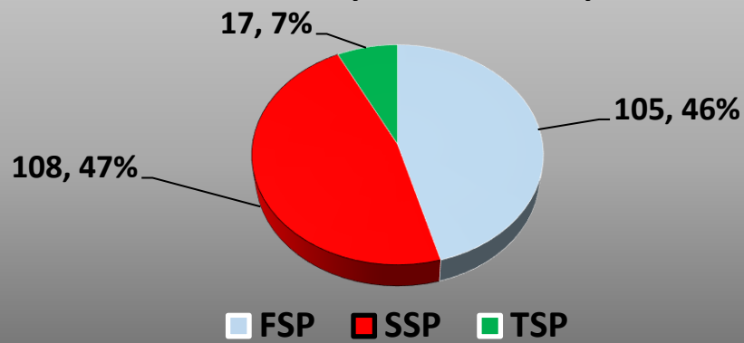
2018 Combined Monthly Total Crashes by Shift
