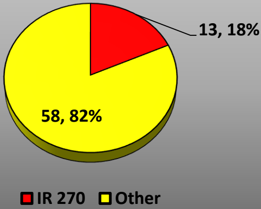
Monthly IR 270 Crashes vs. all other Crash Locations
