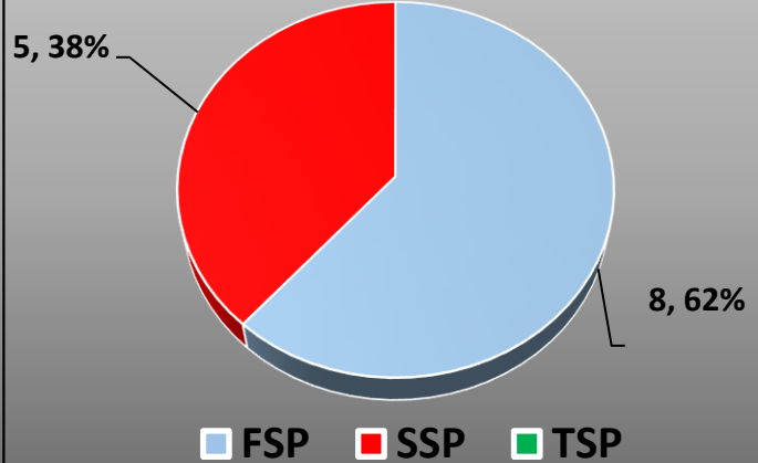
Monthly Total IR 270 Crashes by Shift
