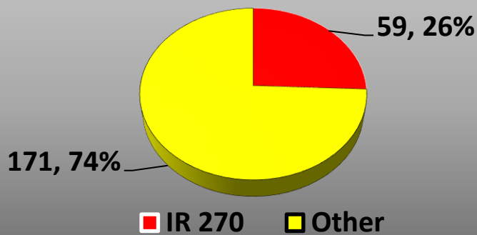
2018 Combined Monthly IR 270 Crashes vs. all other Locations
