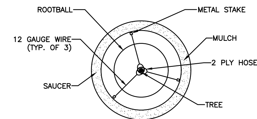
DETAIL 700 - TREE STAKING DETAIL NOT TO SCALE
